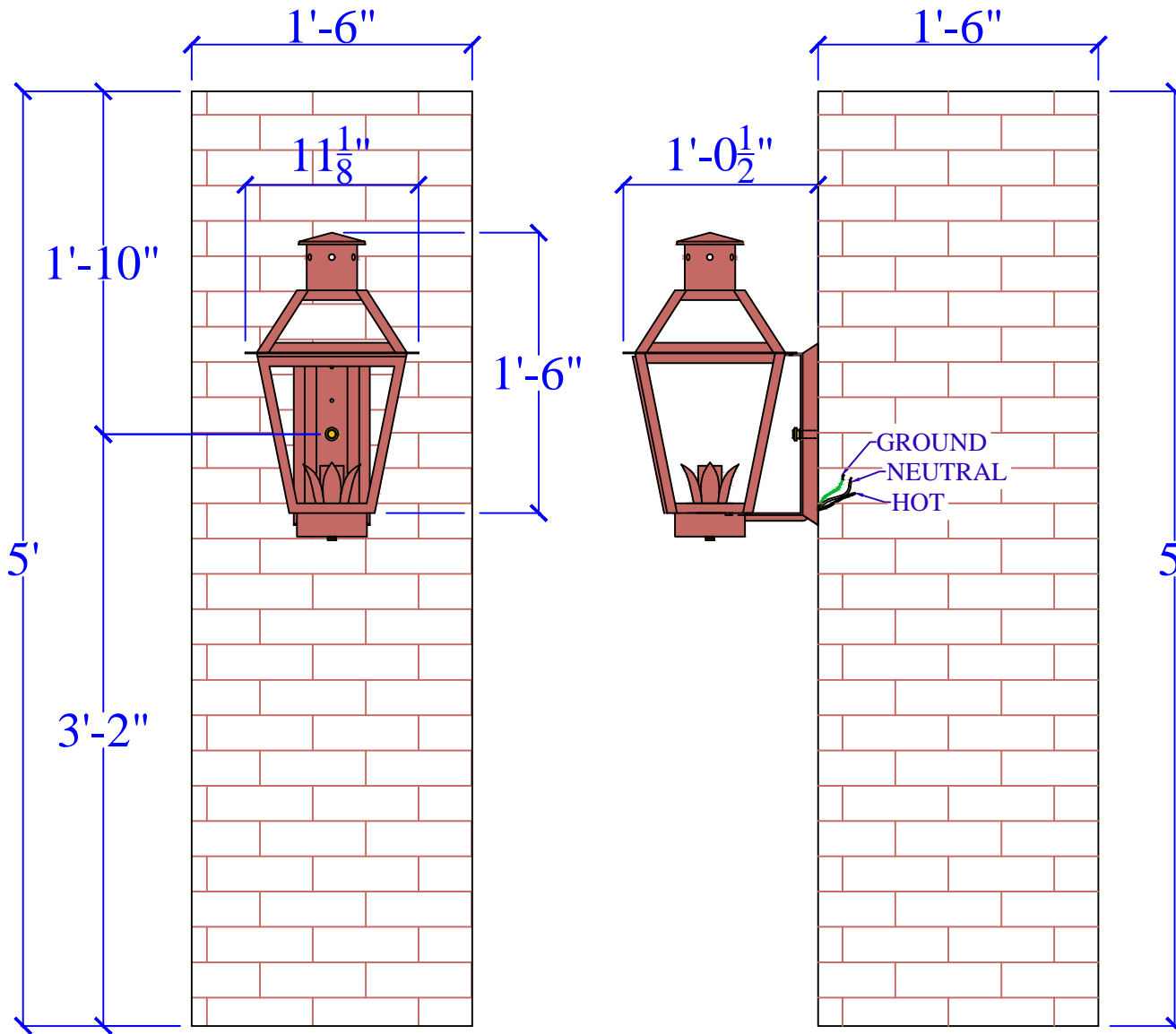
FRONT
