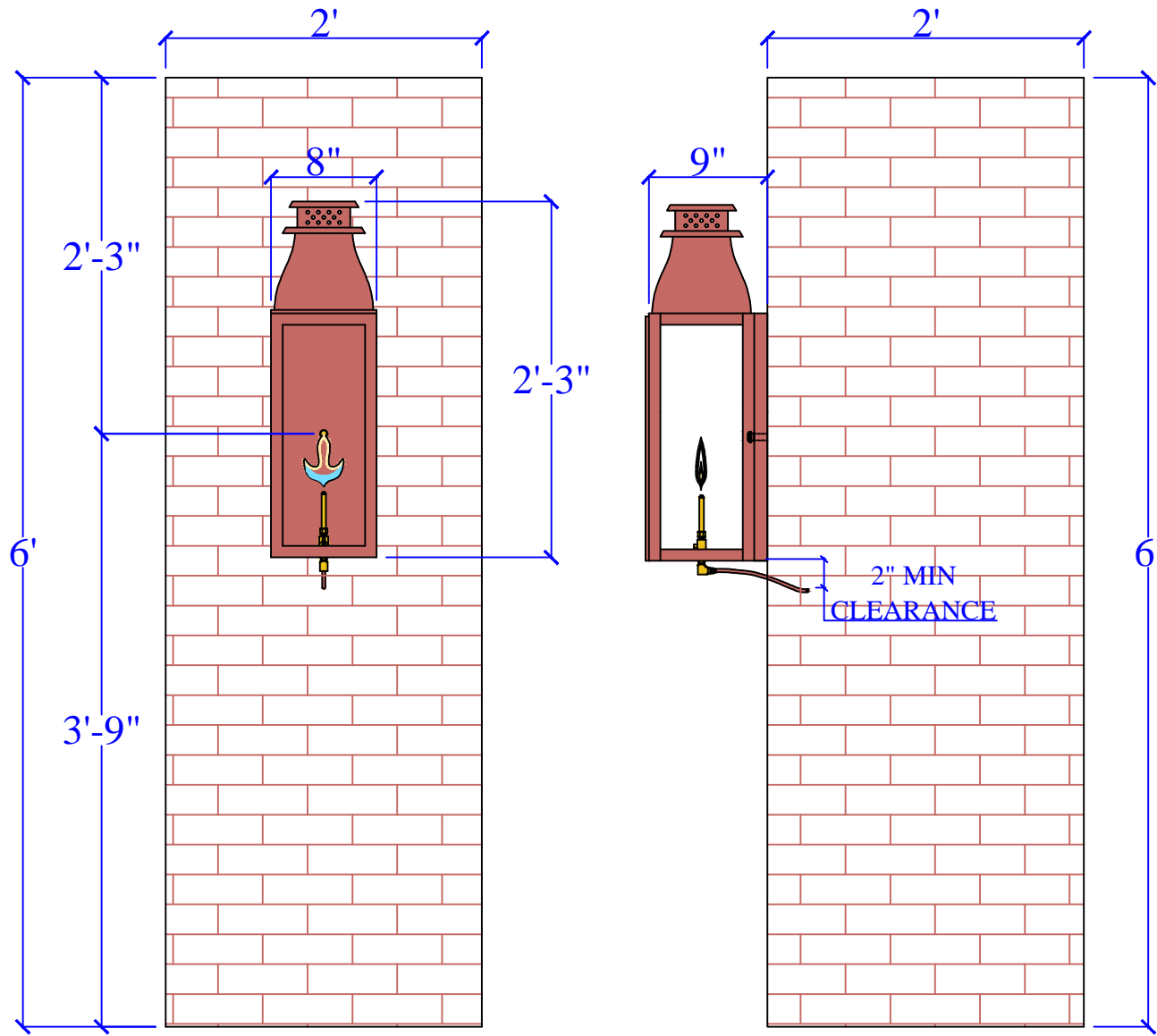
FRONT
